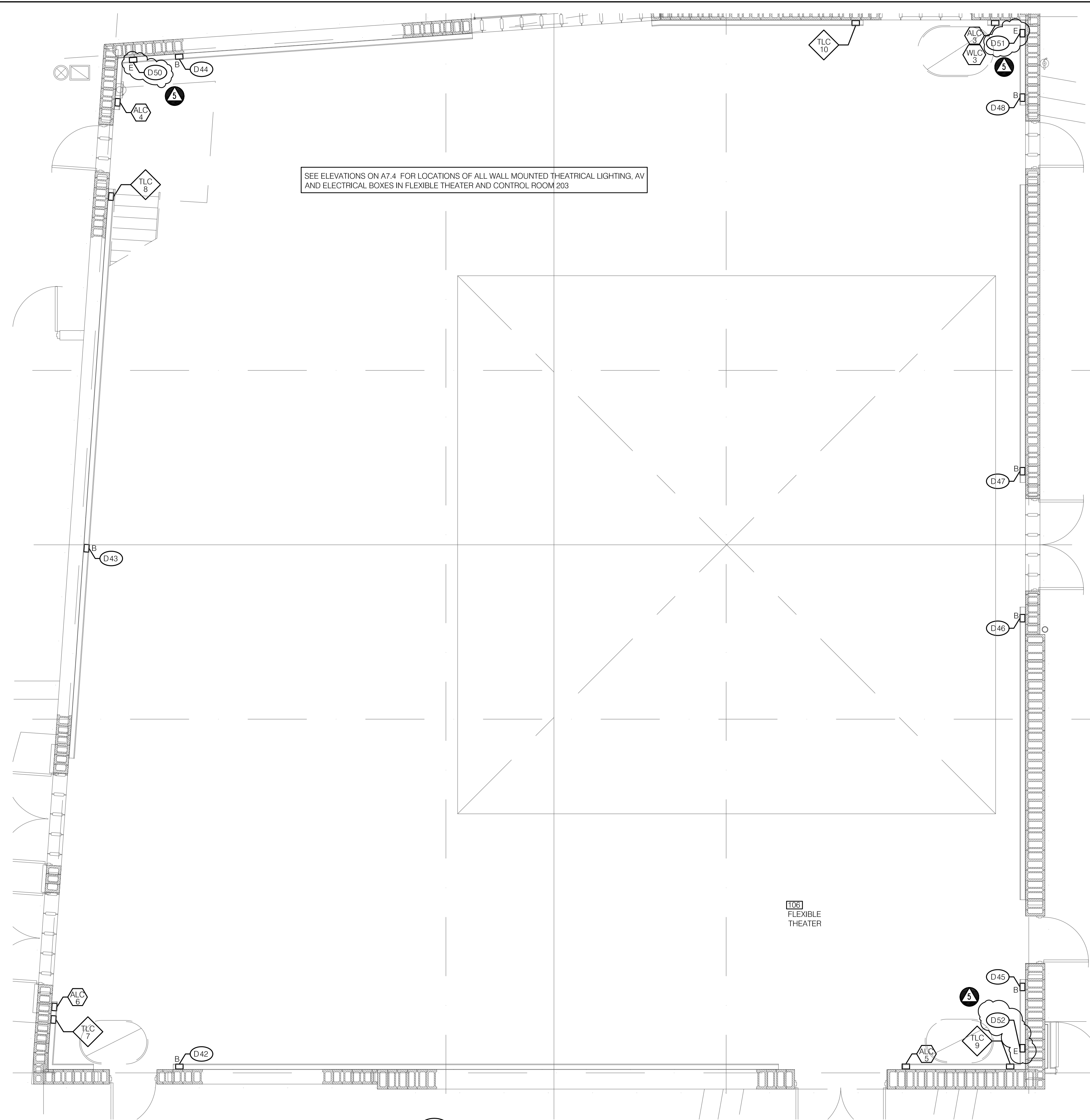
2 MAIN LEVEL THEATER LIGHTING DEVICES TE-1 SCALE: 1/4" = 1'-0"
