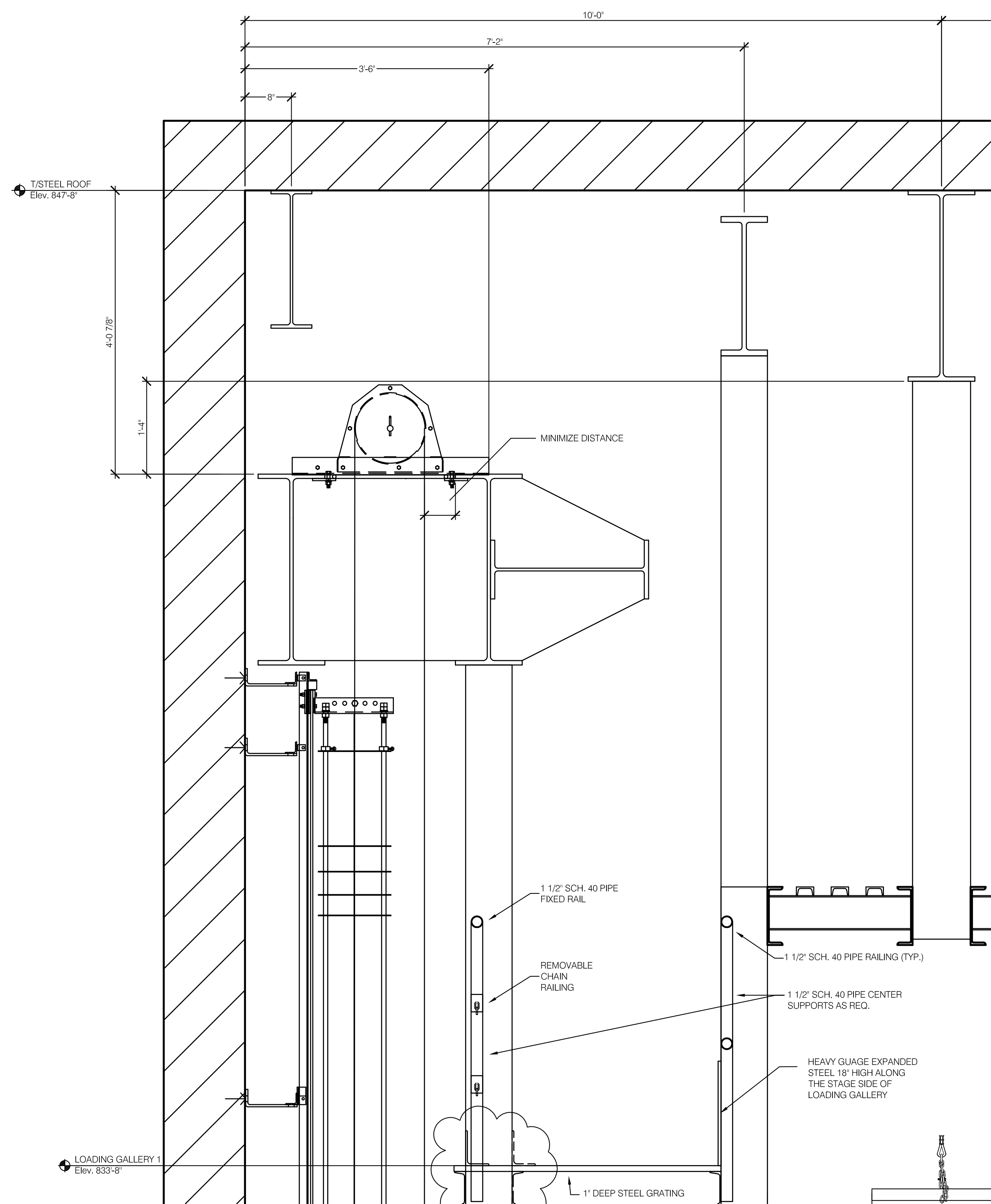
2 HEAD BLOCK STEEL: ELEVATION S-3 SCALE: 1" = 1'-0"
