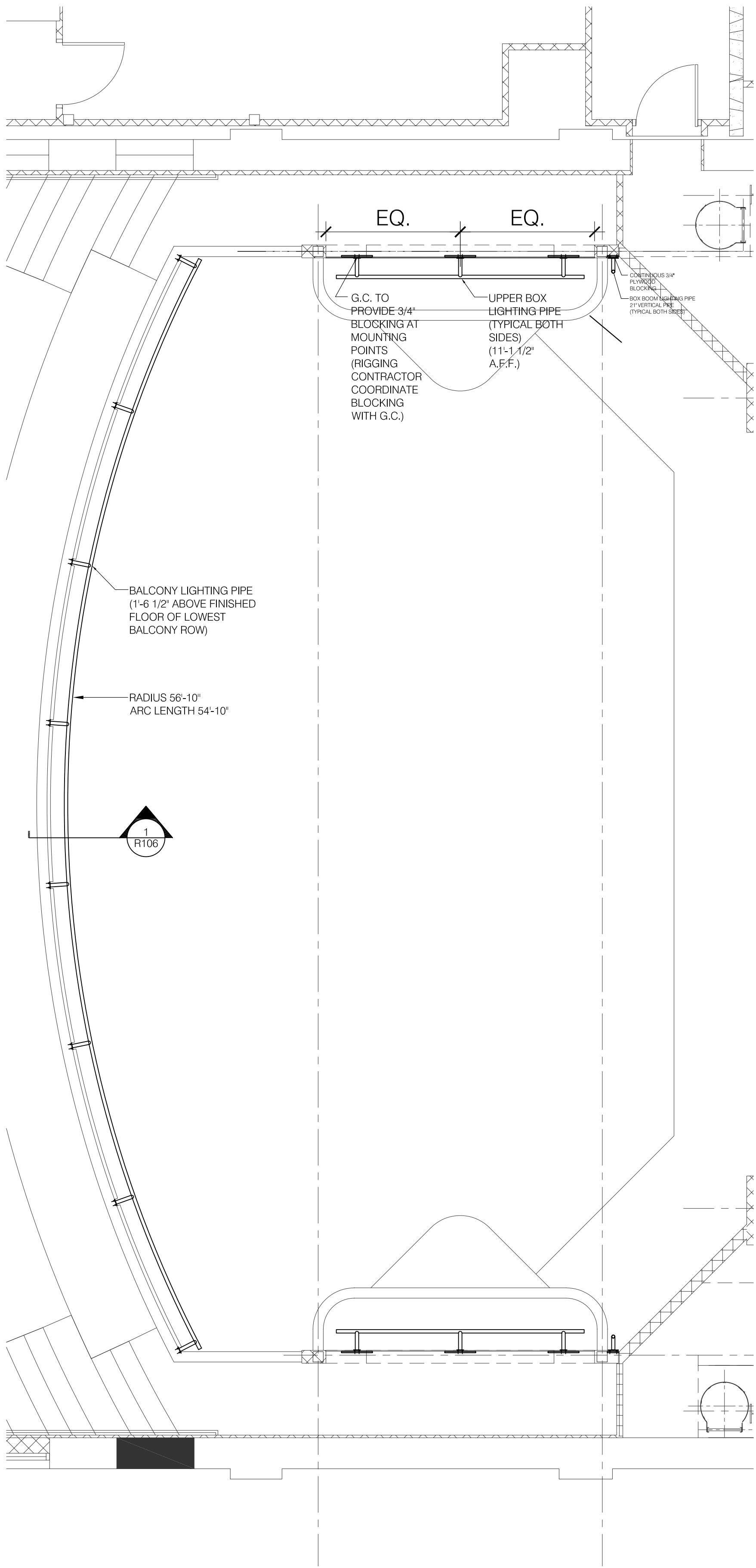
1 THEATER RIGGING 2ND FLOOR - PART PLAN R101
