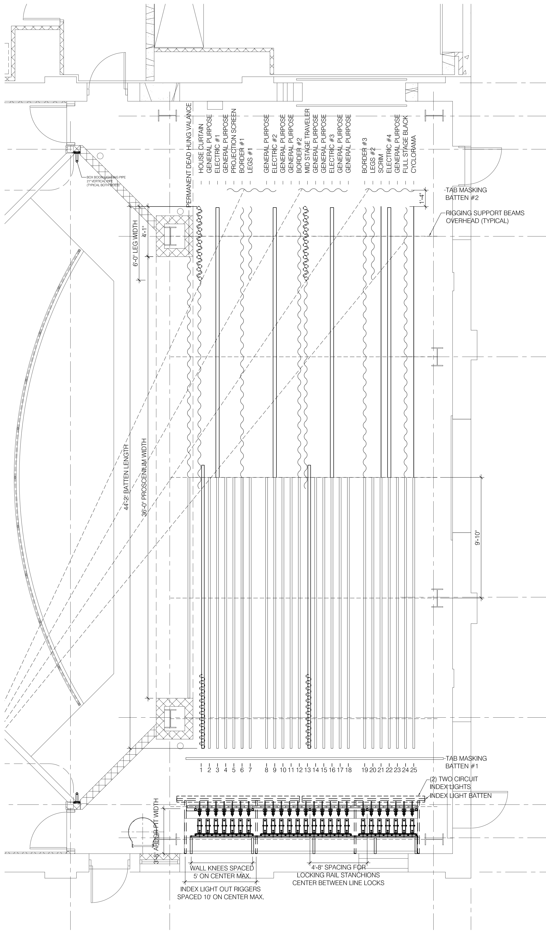
2 THEATER RIGGING BATTEN & DRAPERY - PLAN R101
